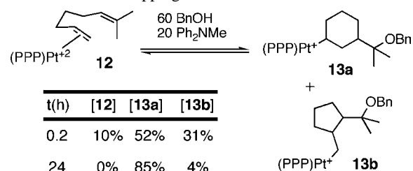
Scheme 1. Trapping of Carbocationic Intermediates
